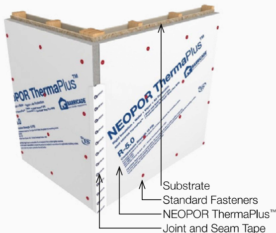
■ Figure 17: Typical Exterior Corner
