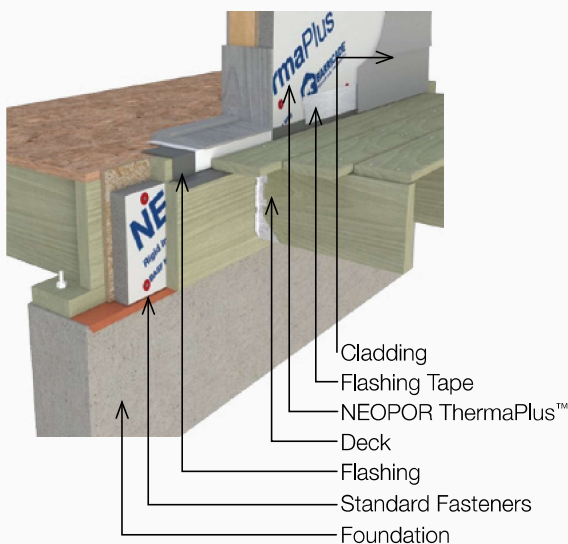
■ Figure 15: Typical Deck/Ledger
