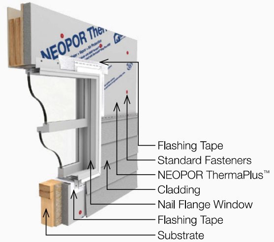
■ Figure 10: Typical Nail Flange Window
