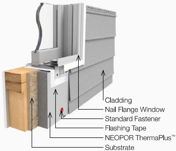
■ Figure 11: Typical Window Sill - Nail Flange Window
