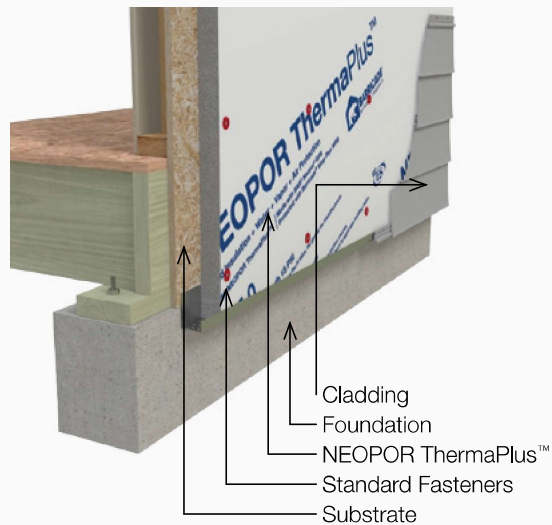
■ Figure 9: Typical Foundation
